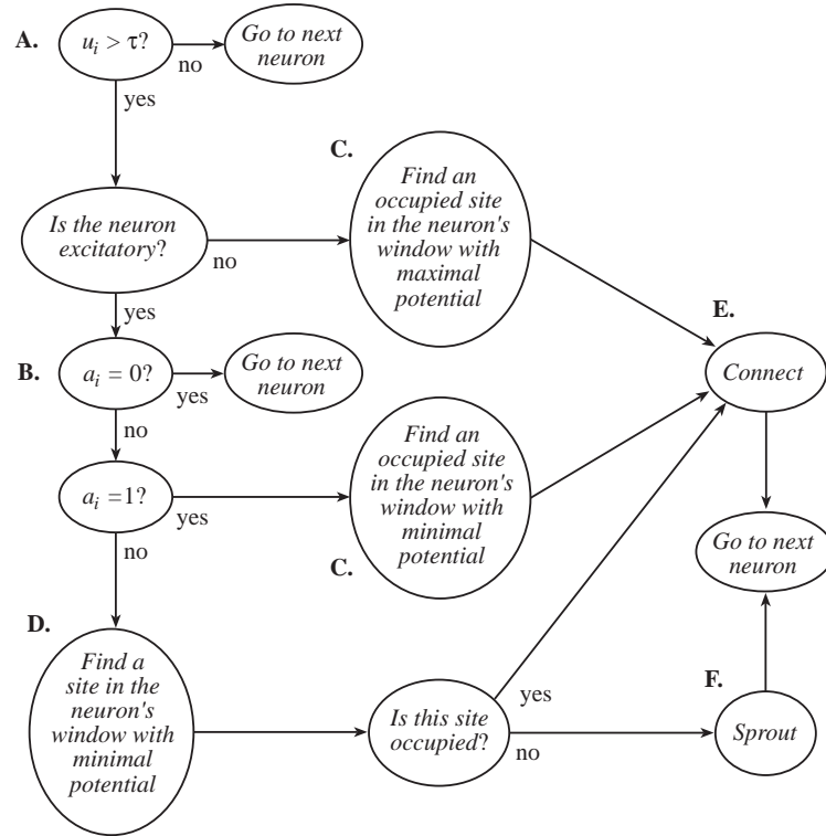
Figure 4: Shown here is the algorithm for the decision to sprout or connect. This is also outlined in section 3.3.
