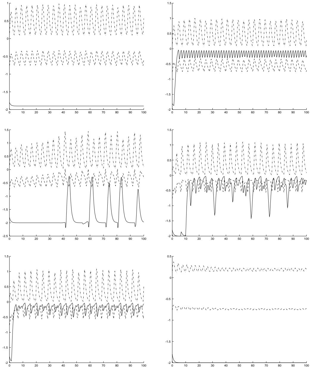
Figure 7: The above six figures show the response of the three mother neurons to an input of strength u_0 = 11 applied at locations a = 7, 9, 11, 13, 15 and 20 . Applying input to any of the locations a \in [1, 7] gives the same response as the first figure and is the same response as the rest state. As well, input applied to any a \in [20, 30] results in the same response as the last figure.
