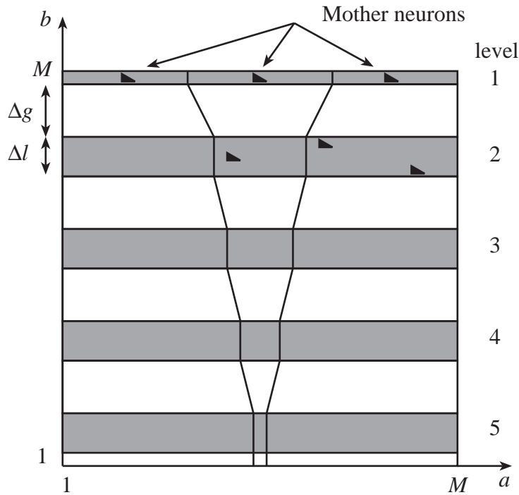
Figure 1: Shown here is the location of the various layers of the network used in the numerical experiments. It depicts the location of the mother neurons, the various levels and the location of the input layer. Also included is the vertical cone extending from an external input located at (a, b) = (15, 1) .
