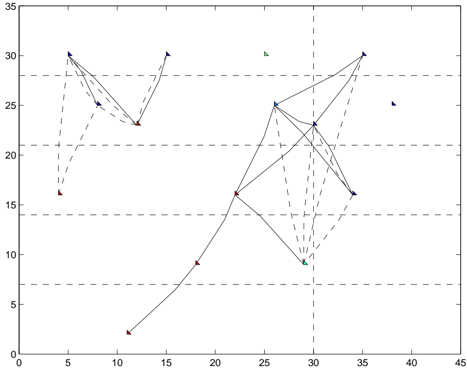
Figure 2: Illustrated above is a sample network showing a few mother neurons along with their children. When a new neuron is created in the i th layer (generation g_i = i ) it is assigned a_i = G + 1 potential axonal connections ( G + 1 - g_i can sprout) and S potential synaptic connections. As the network evolves both of these values can decrease. The horizontal dashed lines divide the net into the five levels while the vertical dashed line indicates where the net wraps around so that the neuron at (35, 30) is another image of the neuron at (5, 30) . Solid connections are excitatory; dashed connections are inhibitive.
